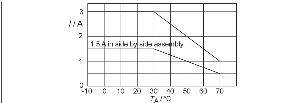
Derating curve for SLO 24TR.
