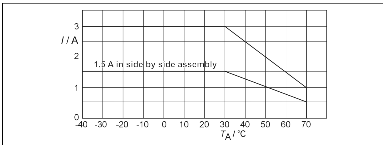
Derating curve for SLO 24CR.
