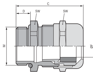
SKINTOP® MS-M ATEX BRUSH
